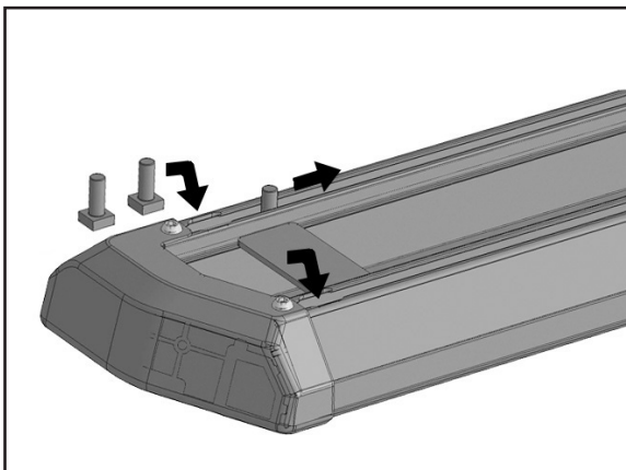
(Figure 9) Slide (3) 8mm T-Bolts into each channel in bottom of Running Board.
