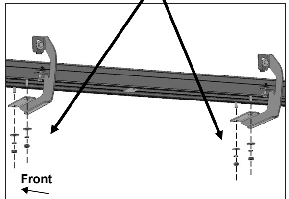
(Figure 11) Attach Running Board to driver/left center and rear Mounting Brackets.
