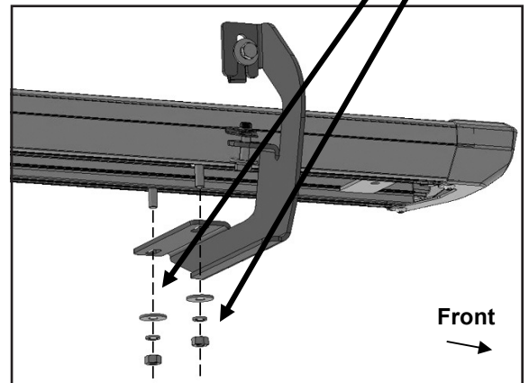
(Figure 10) Attach Running Board to driver/left front Mounting Bracket.
